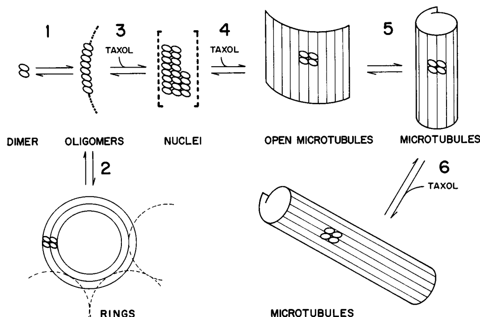
FIGURE 12 Scheme of the \text{Mg}^{2+} -induced self-association processes of GDP-tubulin to form double rings and taxoid-induced microtubules, characterized by time-resolved x-ray scattering. The tubulin dimer, oligomers, ring aggregates, open microtubules, and microtubules (without distinction of their length) have been identified by x-ray scattering in this work. The size and degree of curvature of oligomers are not known from the data, and the microtubule polymerization nuclei (in dashed brackets) have been inferred but have passed undetected.
